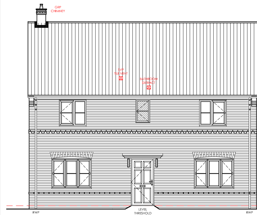
FRONT ELEVATION
