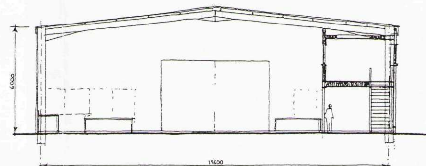
SECTION THROUGH TYPICAL PORTAL FRAME
