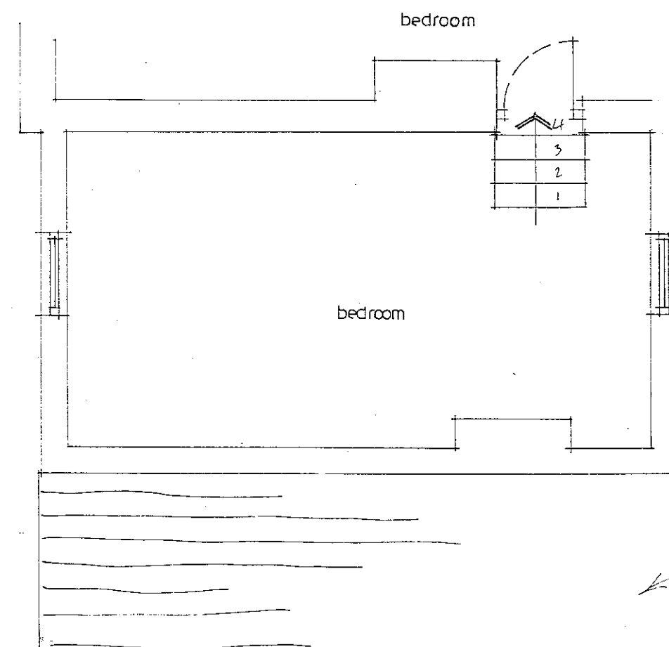
existing first floor part plan 1:50
