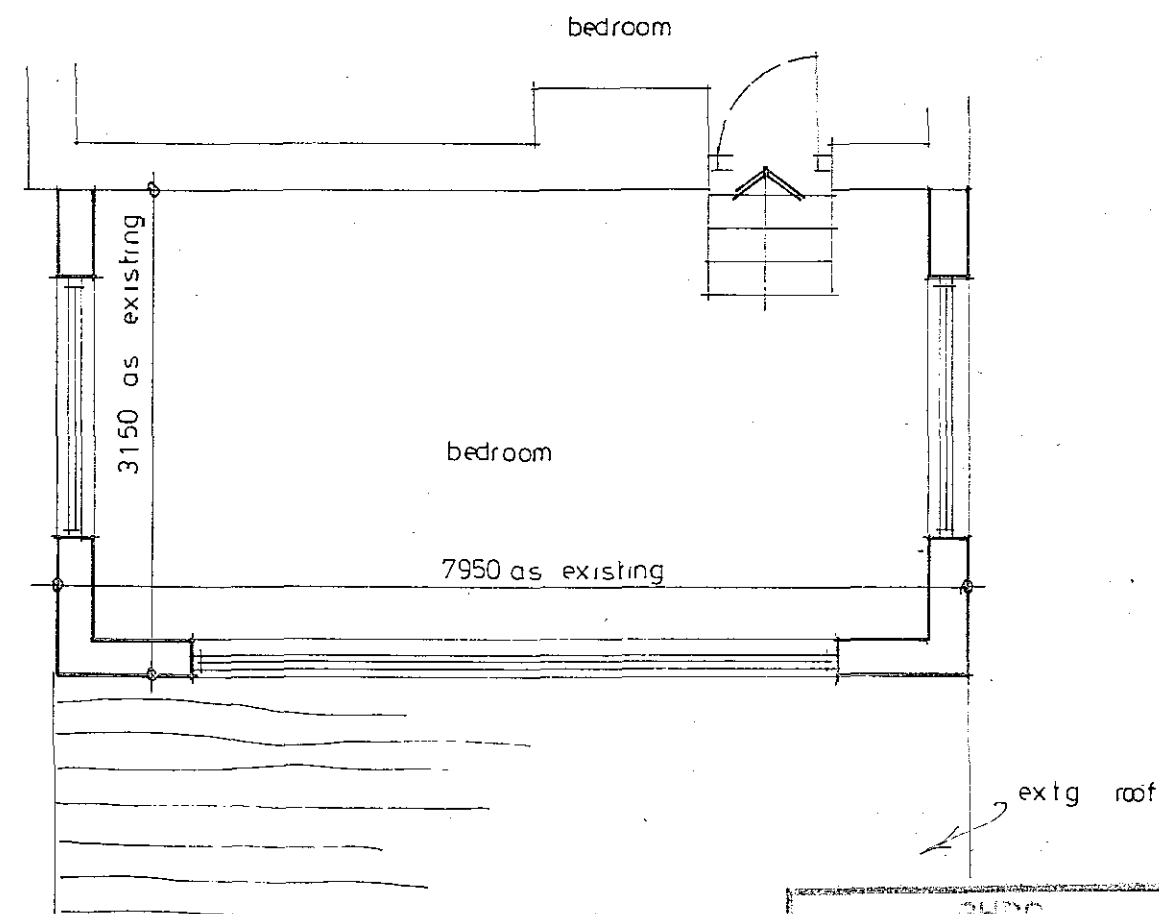
proposed first floor part plan 1:50
