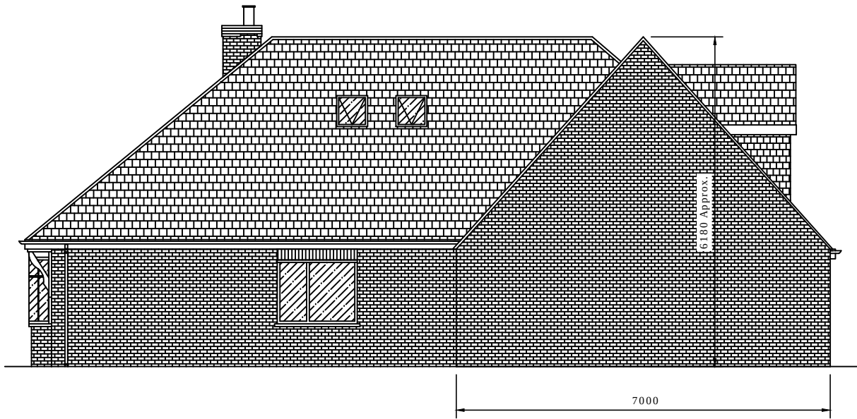
PROPOSED SIDE (EASTERN) ELEVATION
