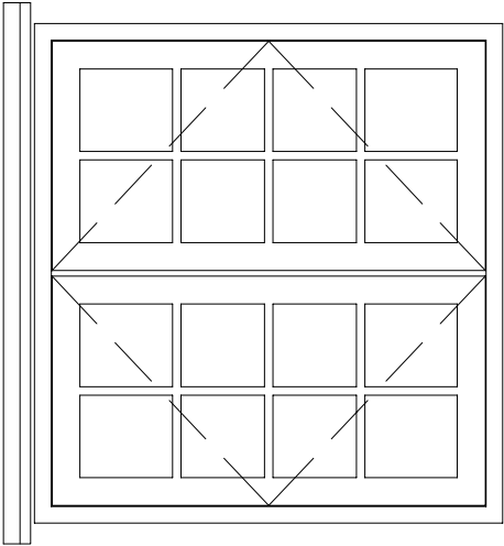
Window Elevation (1:20)
