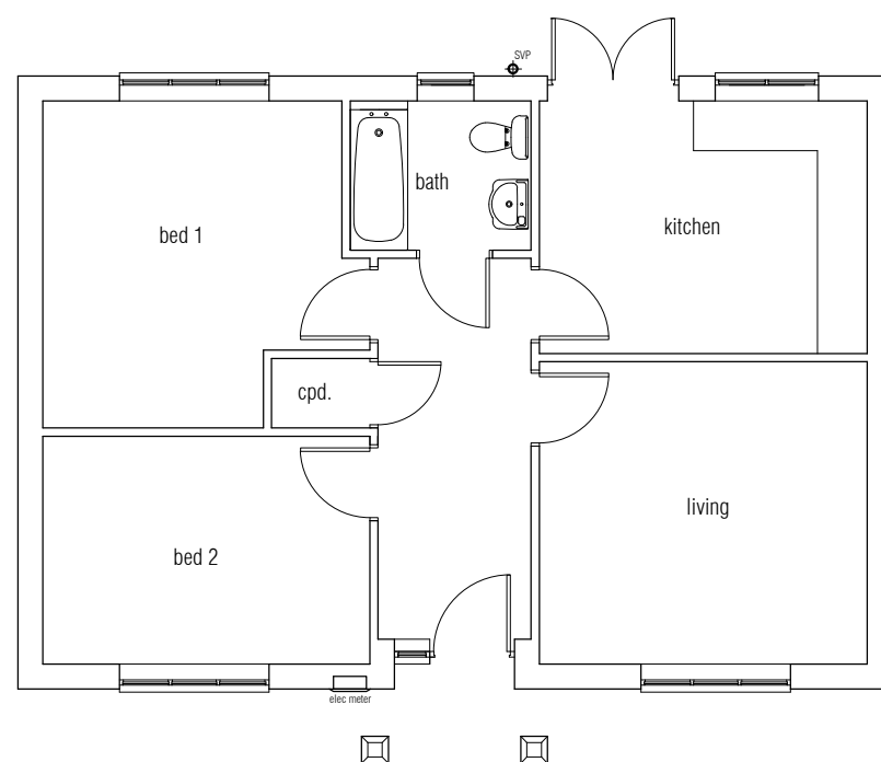
Floor Layout
