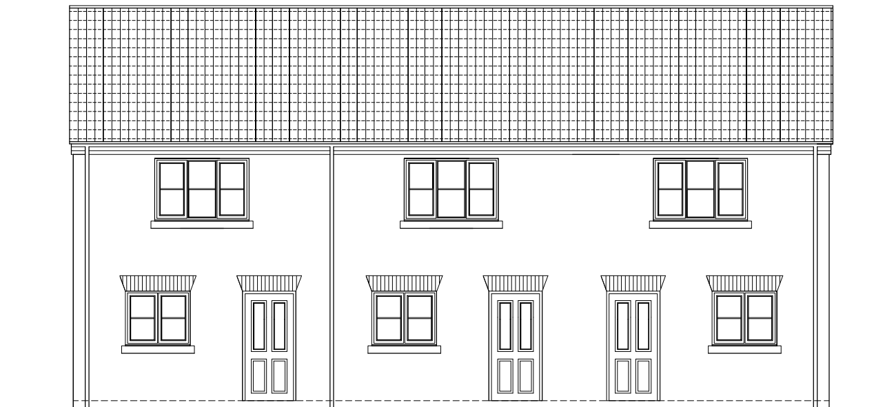
rear elevation
