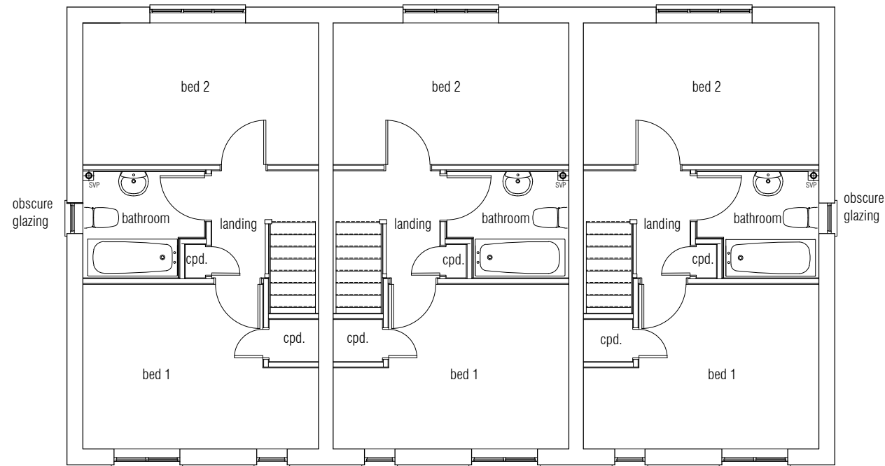
first floor
