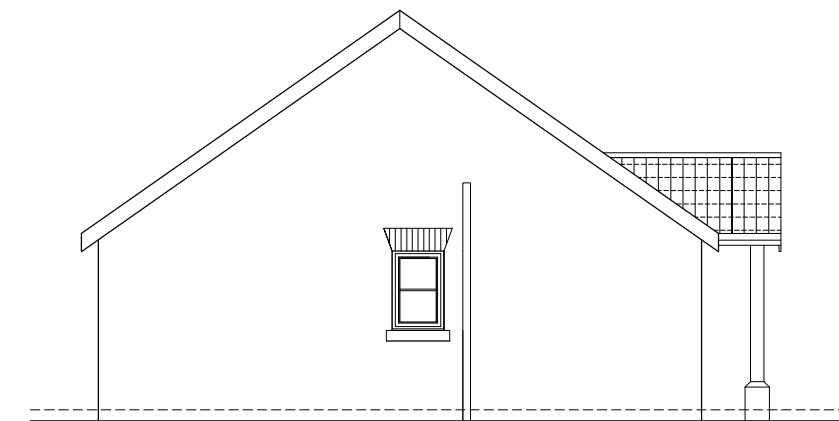
side elevation
