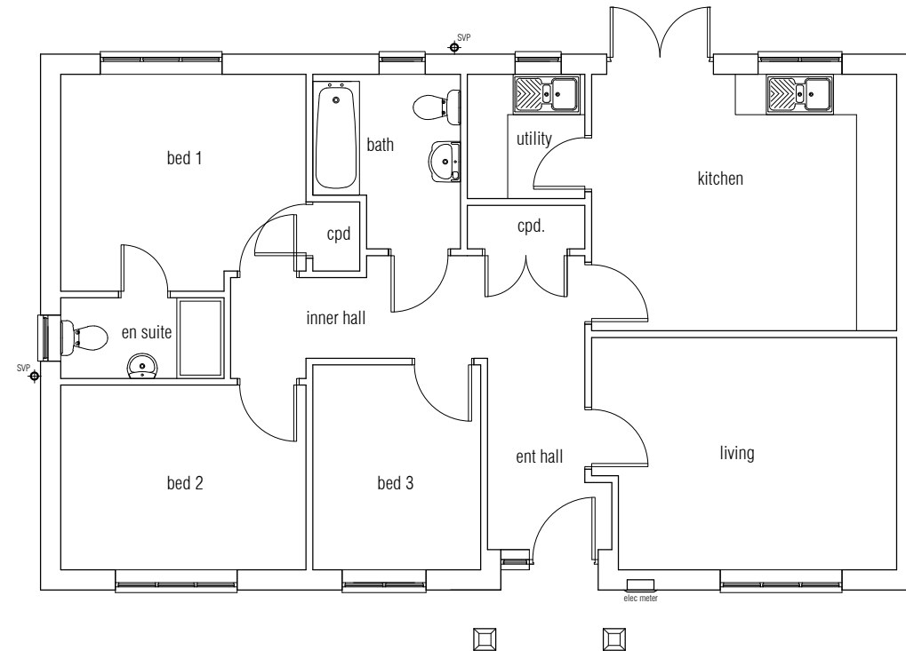
Floor Layout
