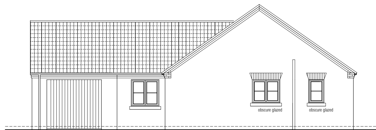
side elevation
