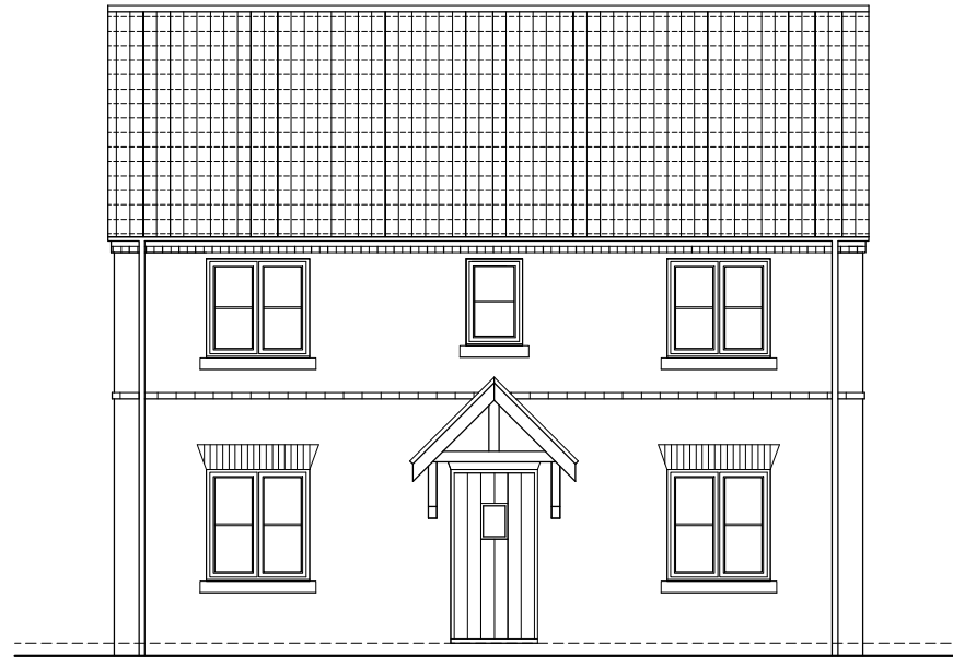
front elevation
