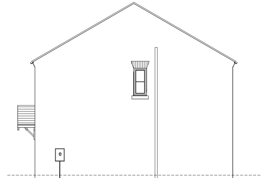
side elevations
