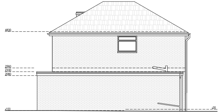
Existing West Elevation Scale 1:50
