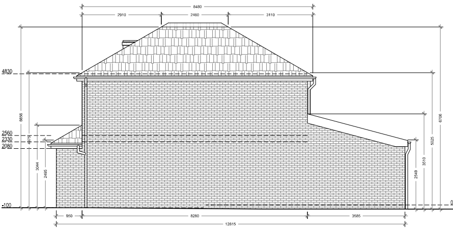
Proposed West Elevation Scale 1:50
