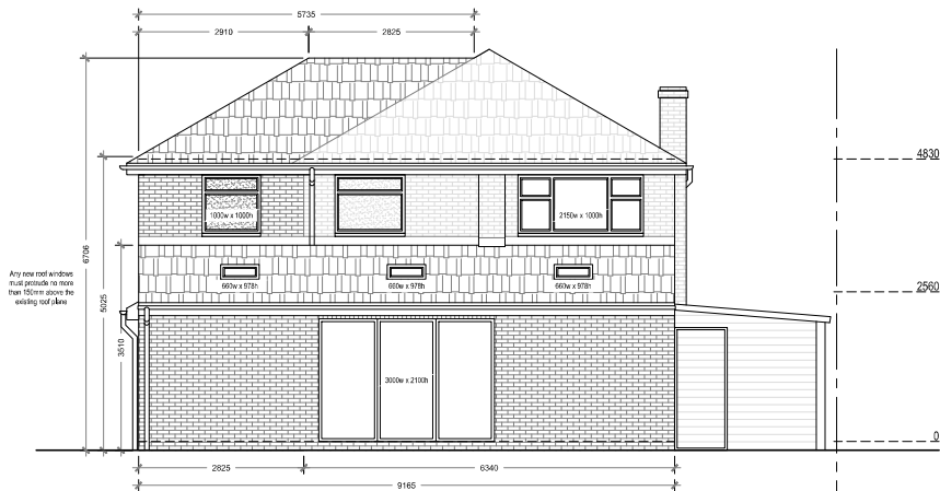
Proposed South Elevation Scale 1:50
