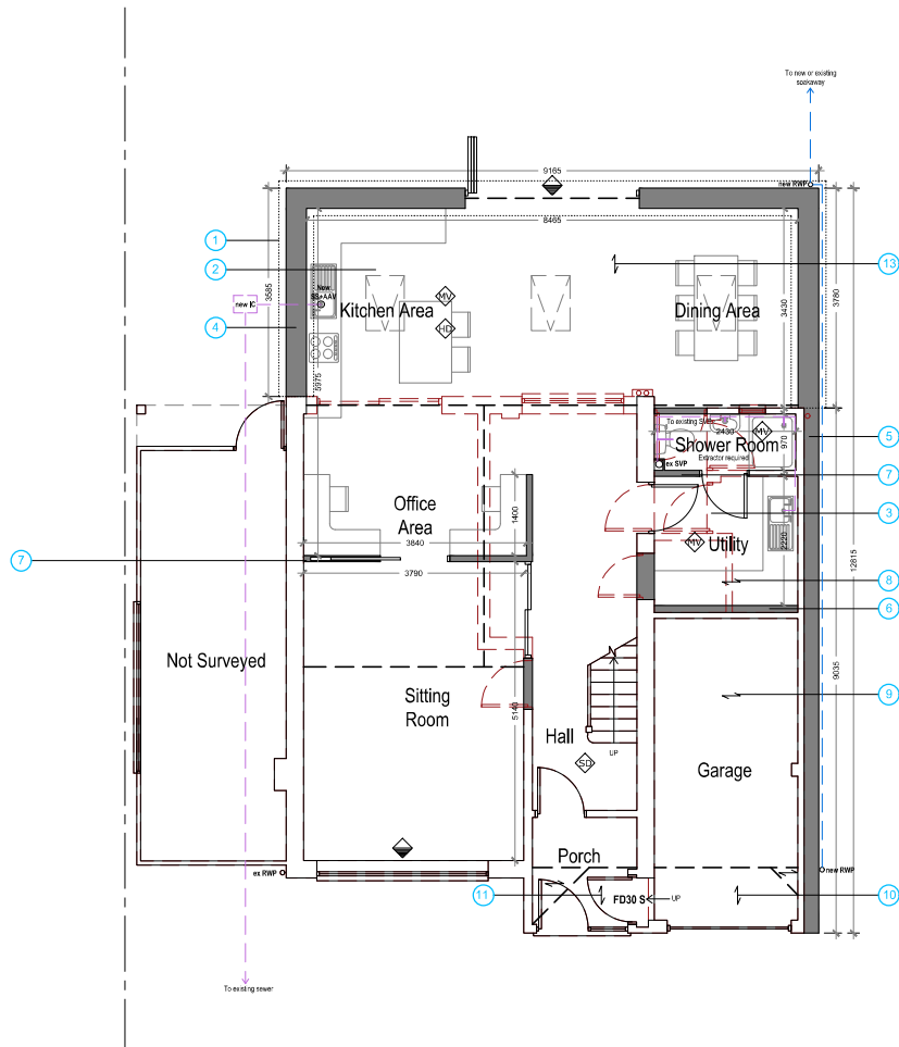
Proposed Ground Floor Plan Scale 1:50 Area ca. 84.91 m 2 Additional area ca. 29.58 m 2
