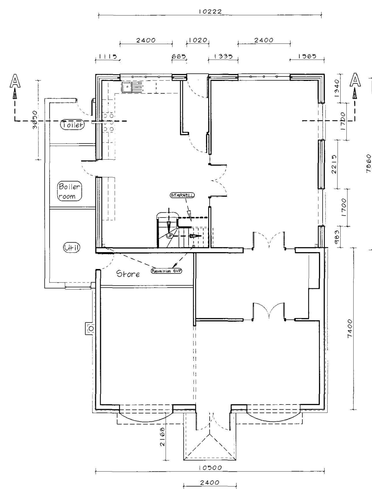
GROUND FLOOR 100:1
