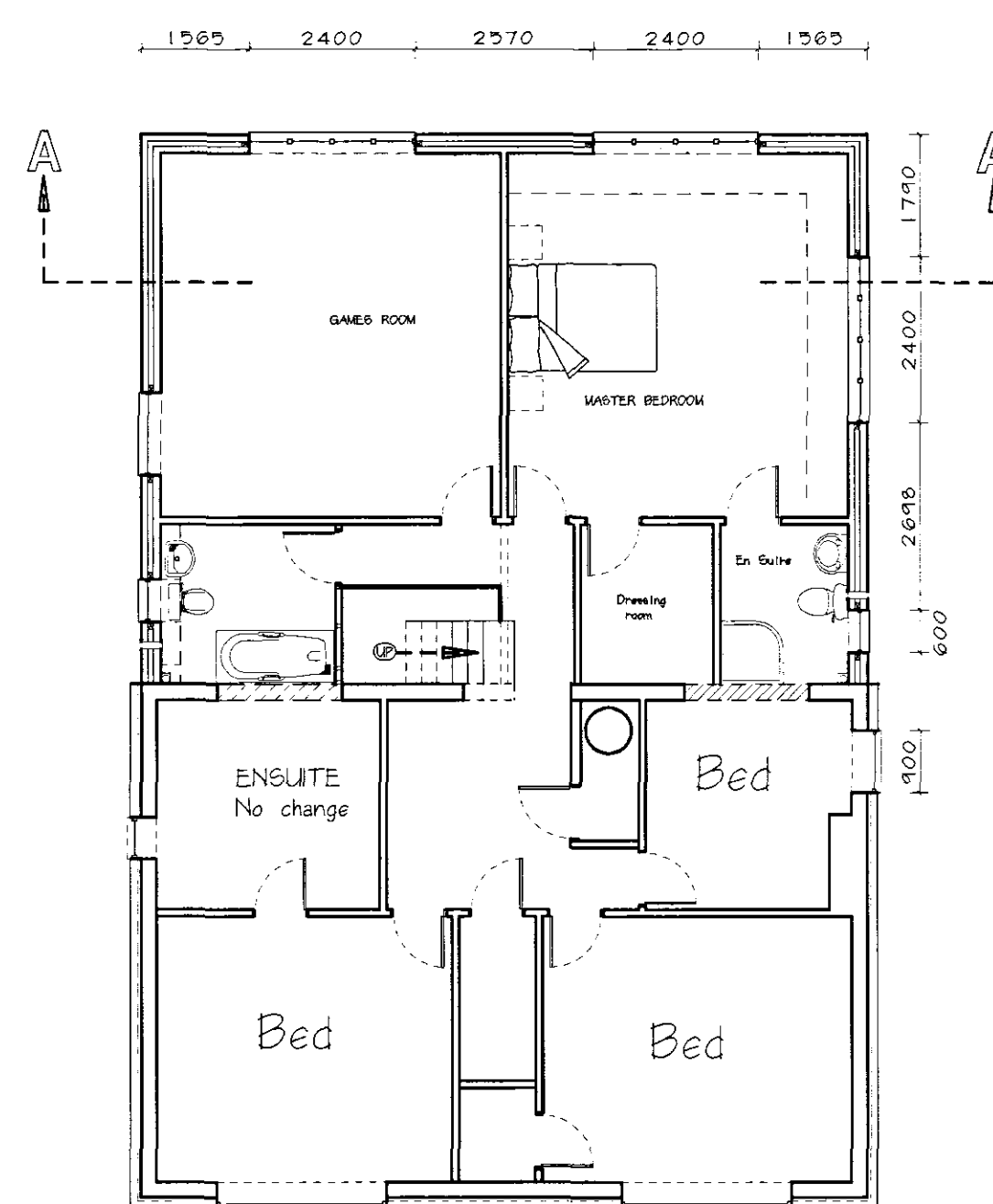
FIRST FLOOR 100:1
