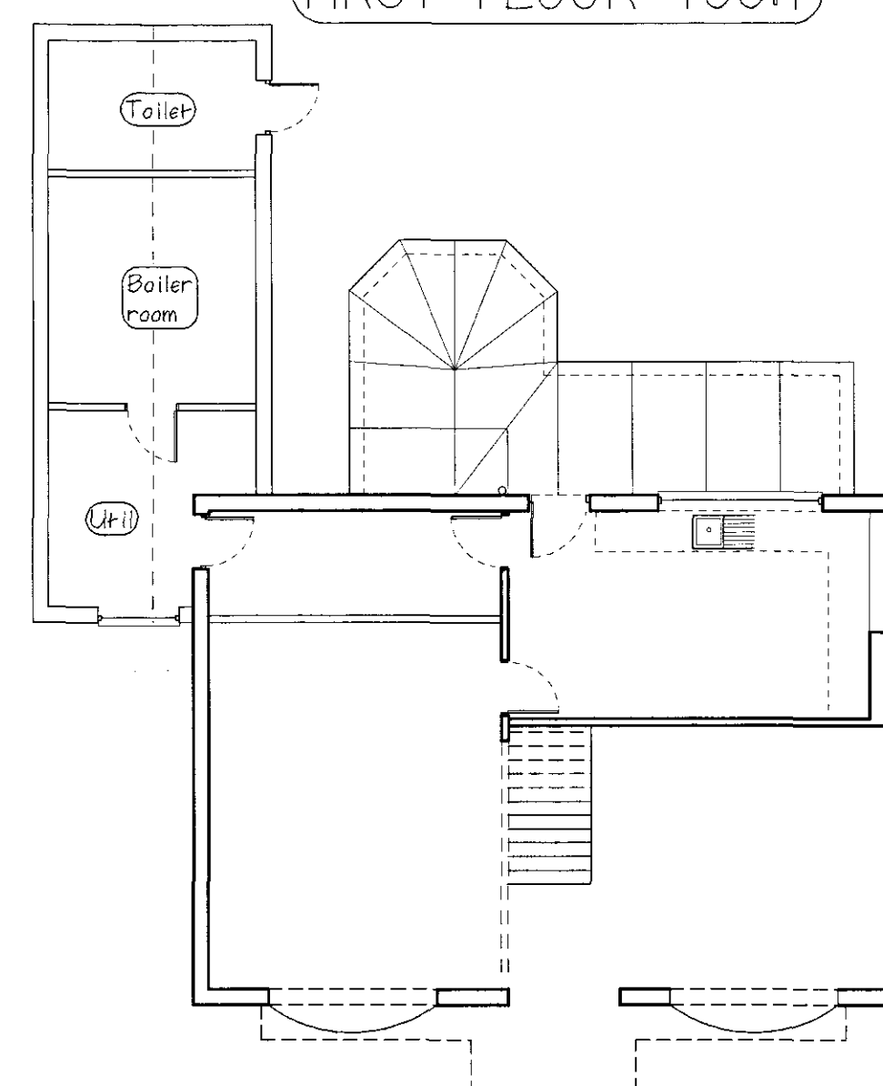
GROUND FLOOR 100:1
