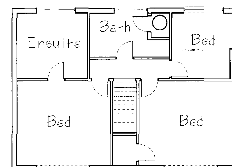
FIRST FLOOR 100:1
