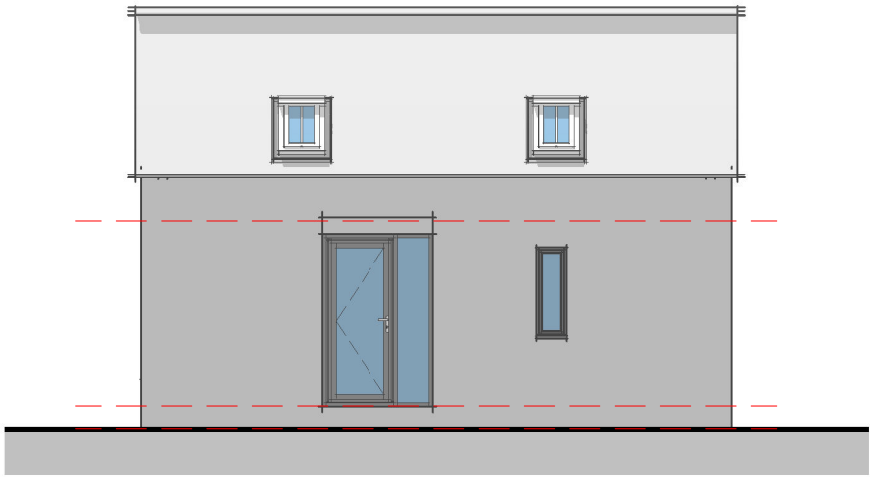
Elevation 03 - Rear 1 : 100
