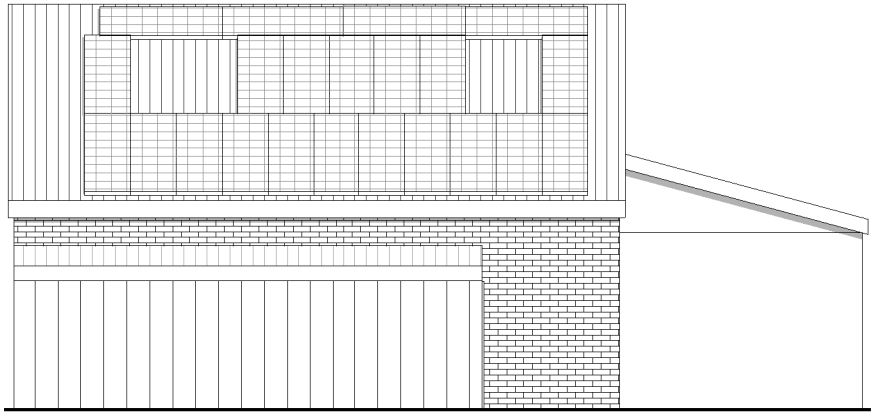
1 Existing Rear 1 : 100
