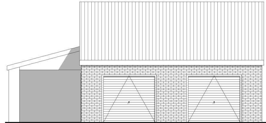
1 Existing Front 1 : 100
