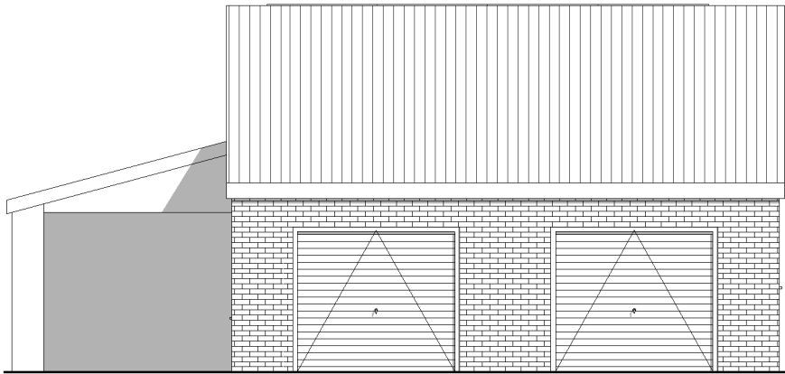
2 Proposed Front 1 : 100
