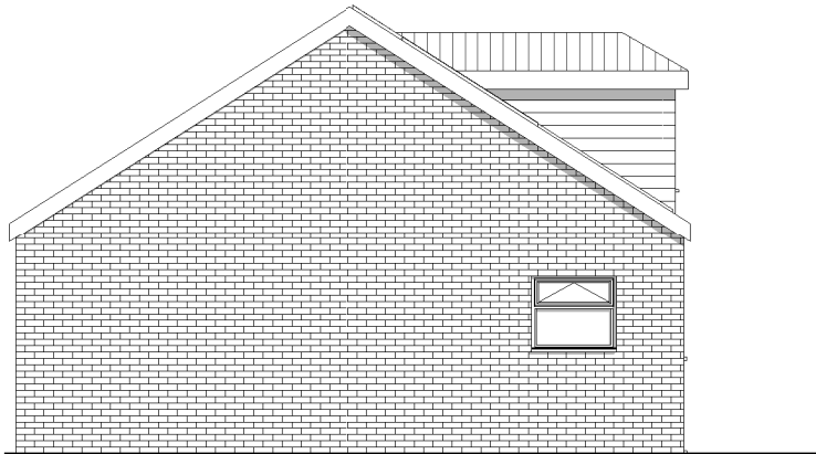
4 Proposed Side A 1 : 100
