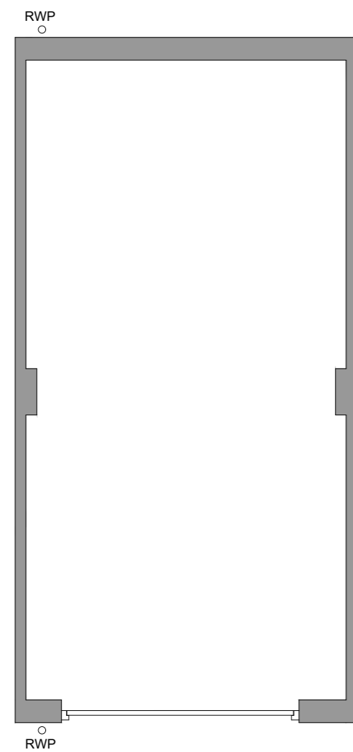
Floor Plan
