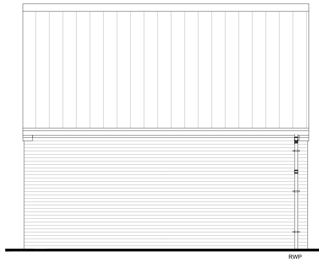
Rear Elevation
