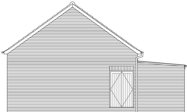
Existing north elevation 1:100
