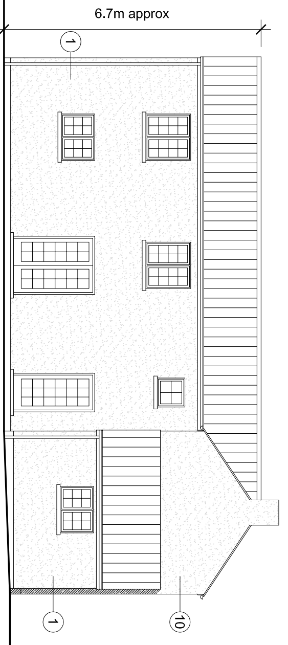
South Elevation (1:100)
