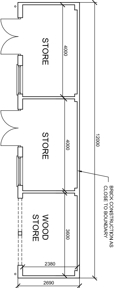
STORAGE BUILDING (28 sq metre internal)
