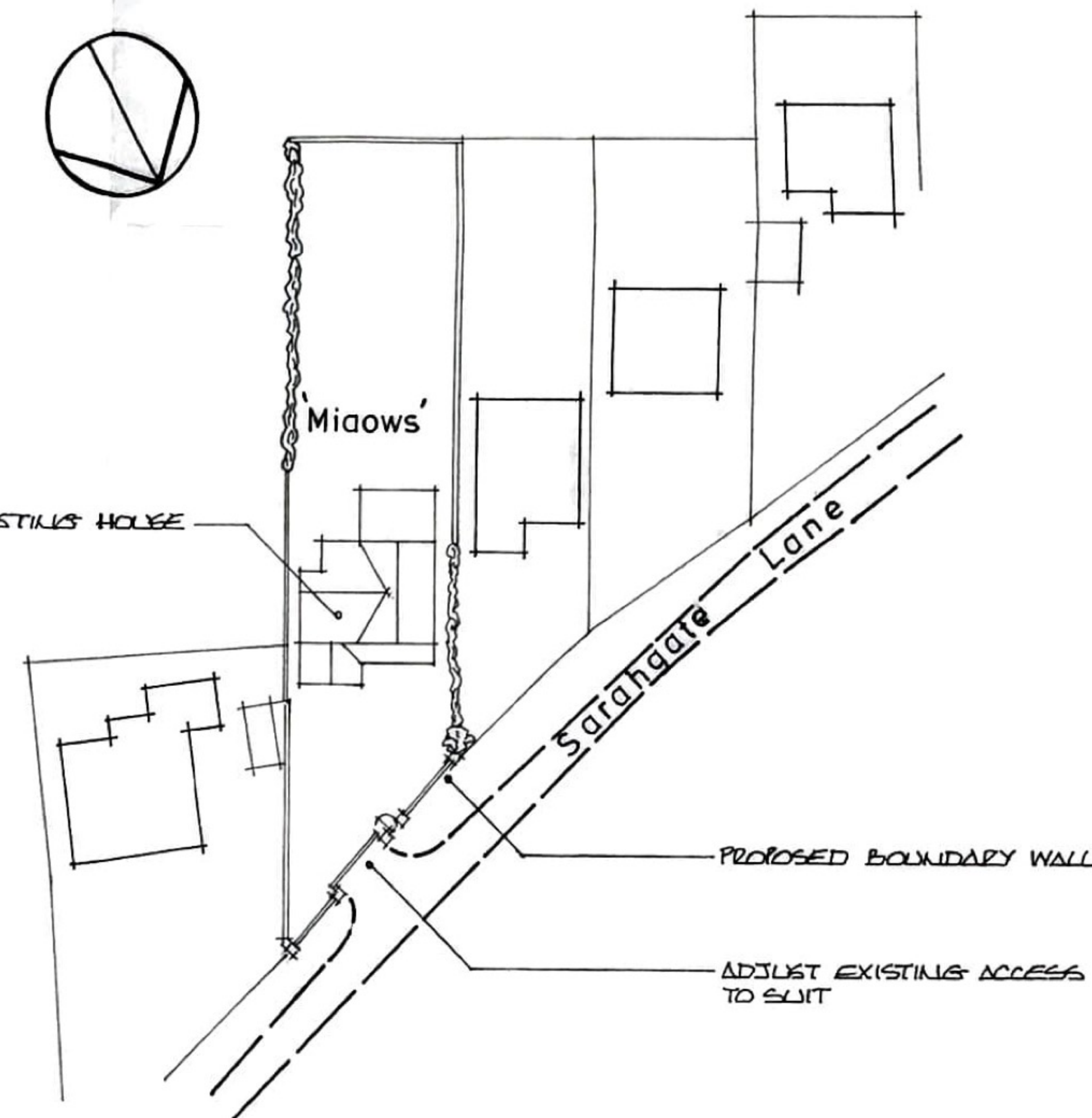
BLOCK PLAN
