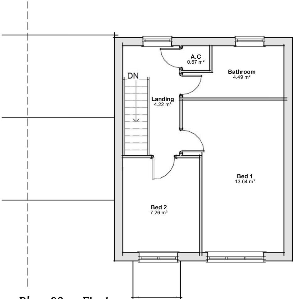
Plan 02 – First 1 : 75
