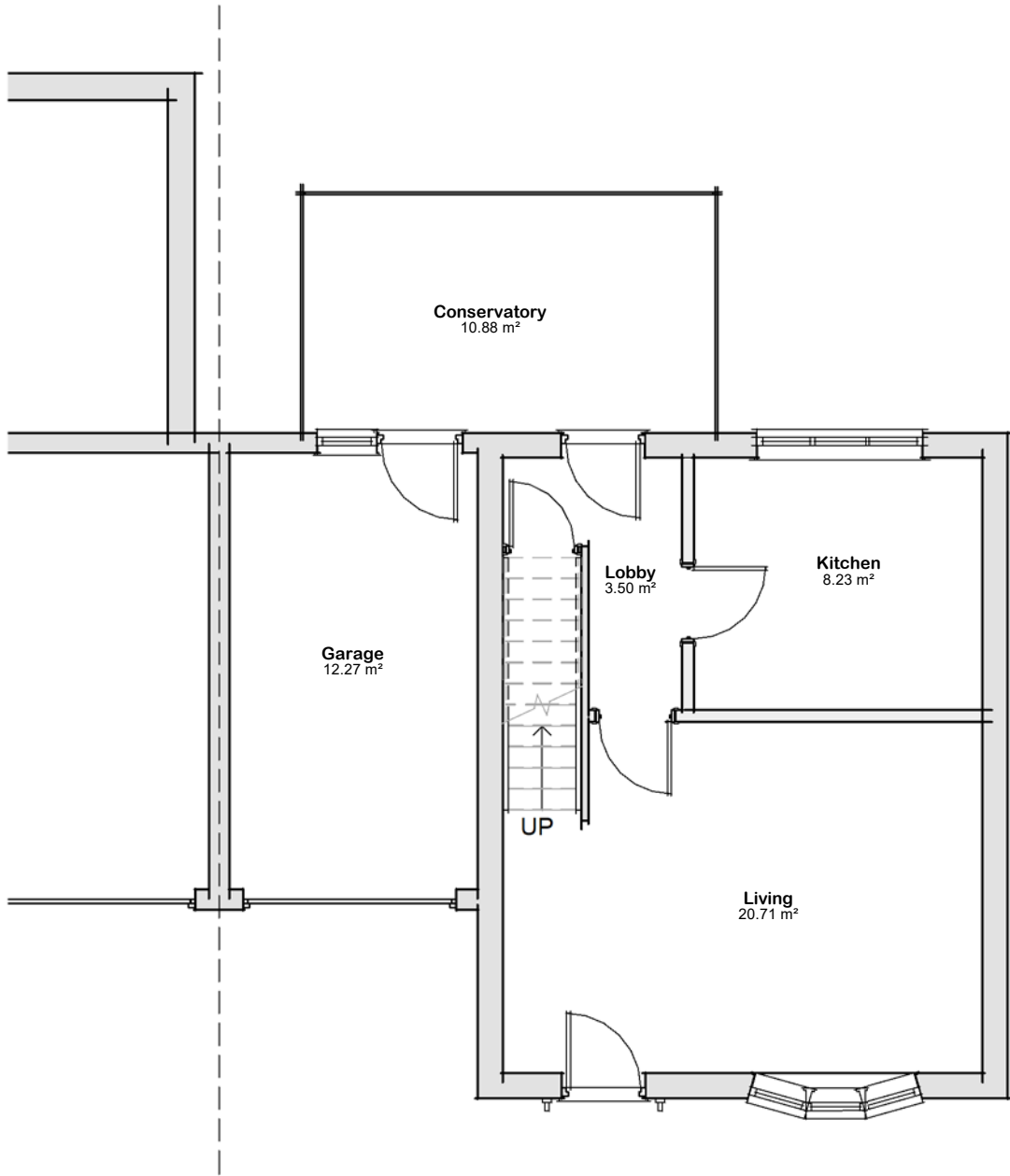
Plan 01 – Ground 1 : 75
