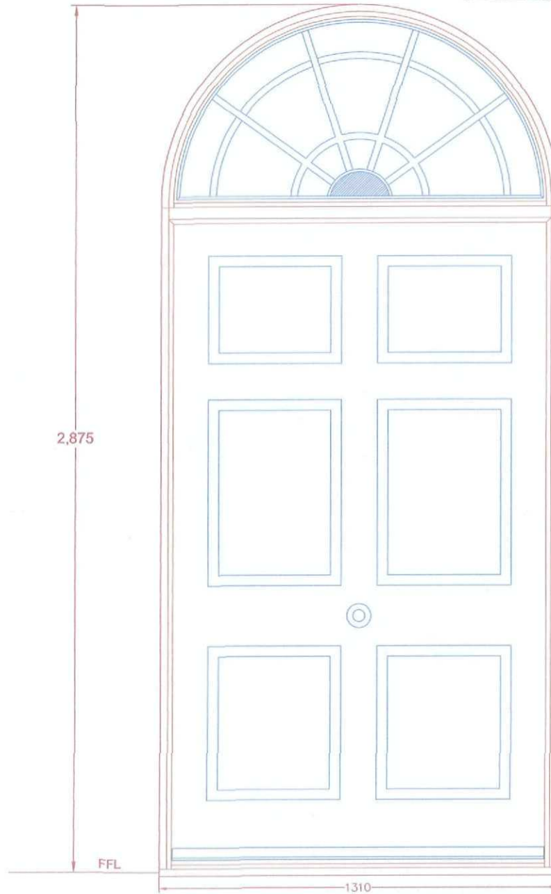
East - D1 Inward opening Option 2
