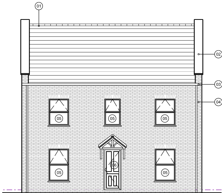
South West Elevation
