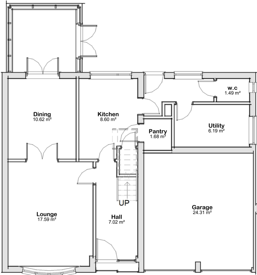
Plan 01 - Ground 1 : 100
