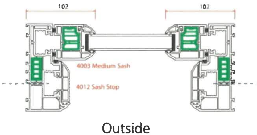
Horizontal section through bottom sash
