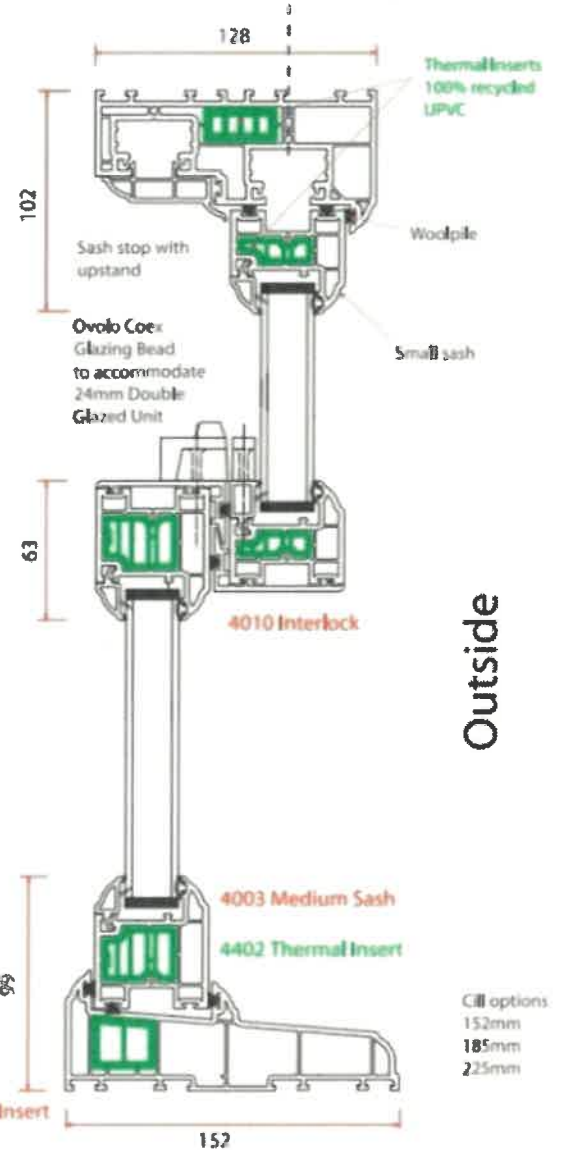
Vertical section through sash
