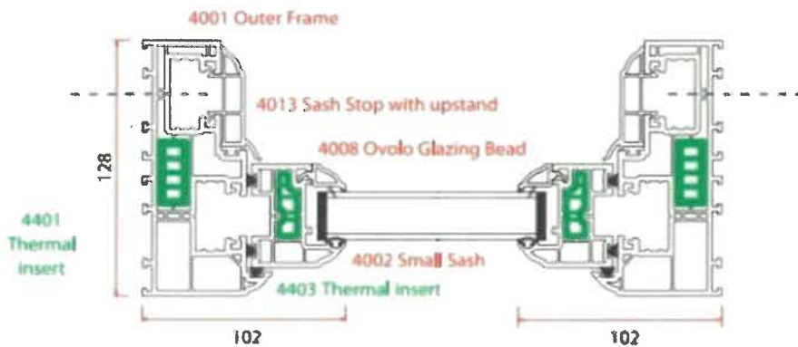
Horizontal section through top sash
