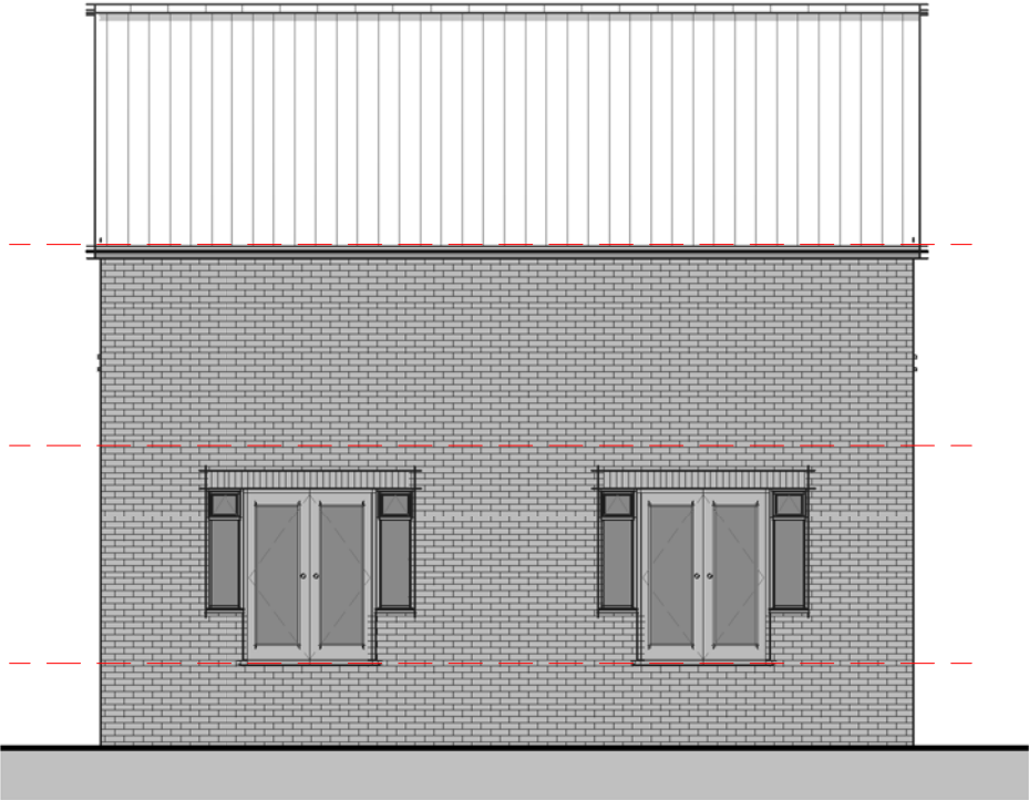
Elevation 03 - Rear 1 : 100
