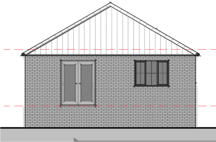
Elevation 03 - Rear 1 : 100
