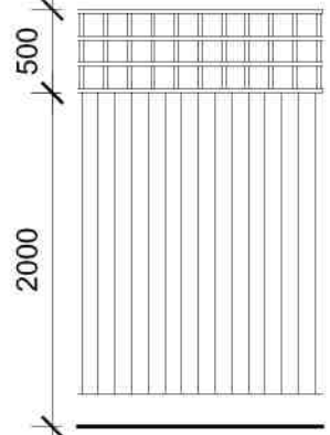
Close Boarded / Trellis Fence
