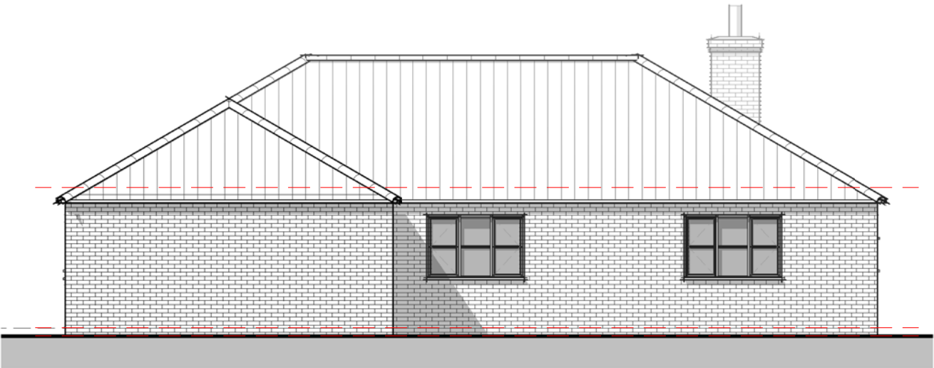
Elevation 03 – Rear 1 : 100
