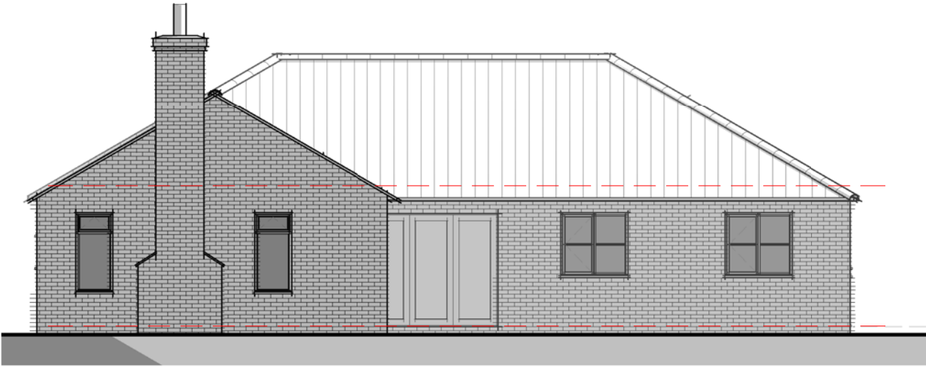
Elevation 01 – Front 1 : 100
