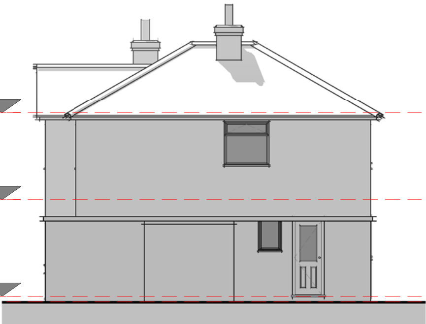
Elevation 02 – Right 1 : 100
