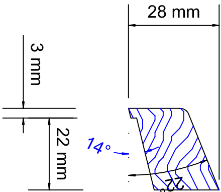
Bottom Sash Bead
