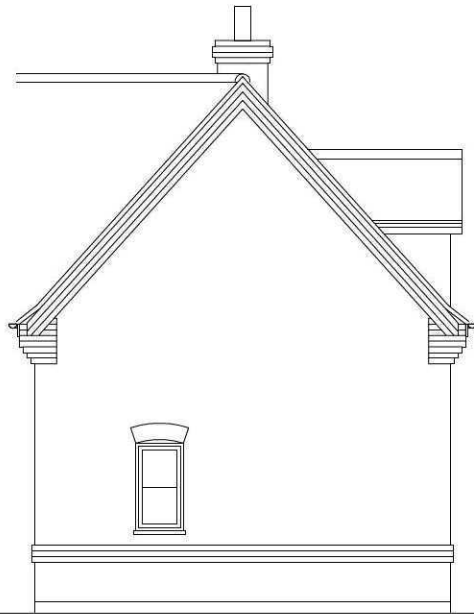
Part East Elevation
