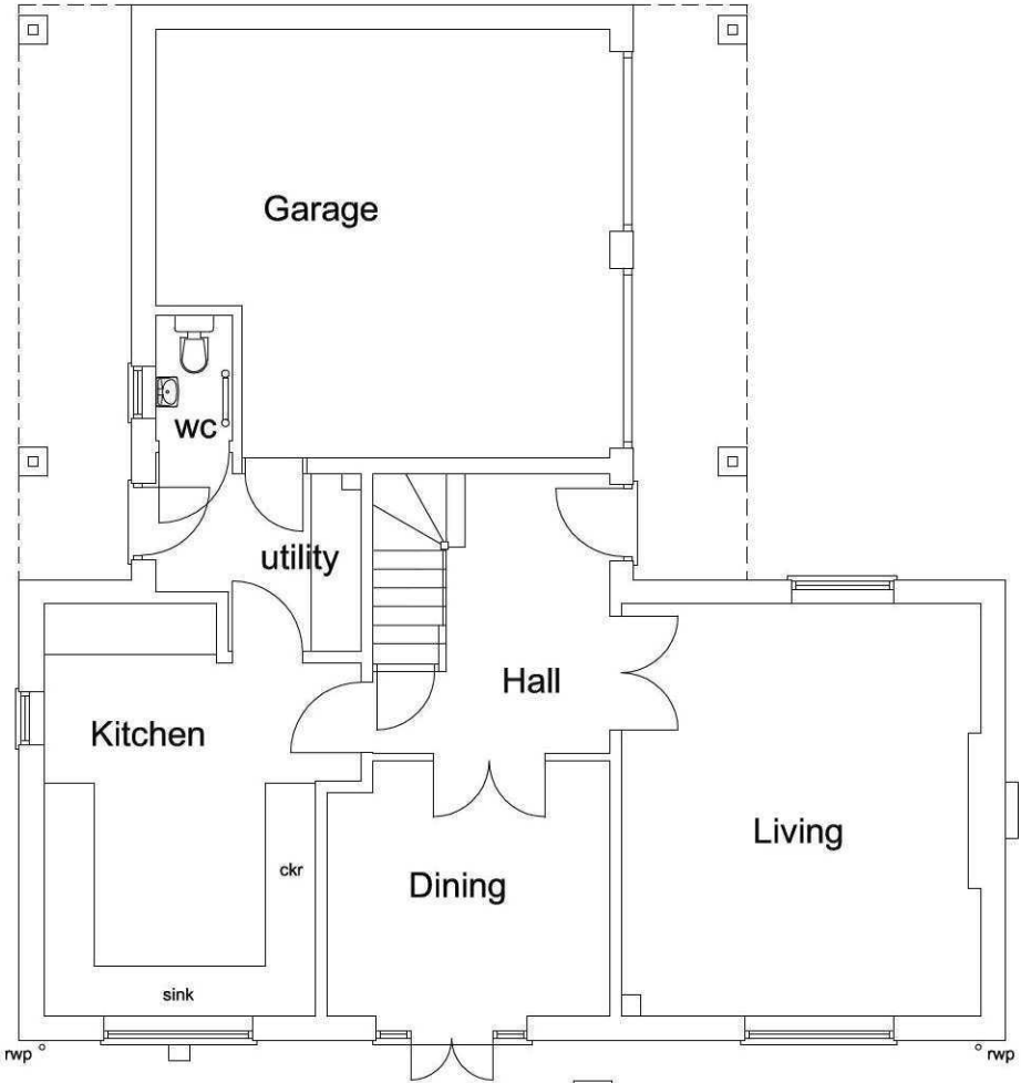
Ground Floor Plan As Existing
