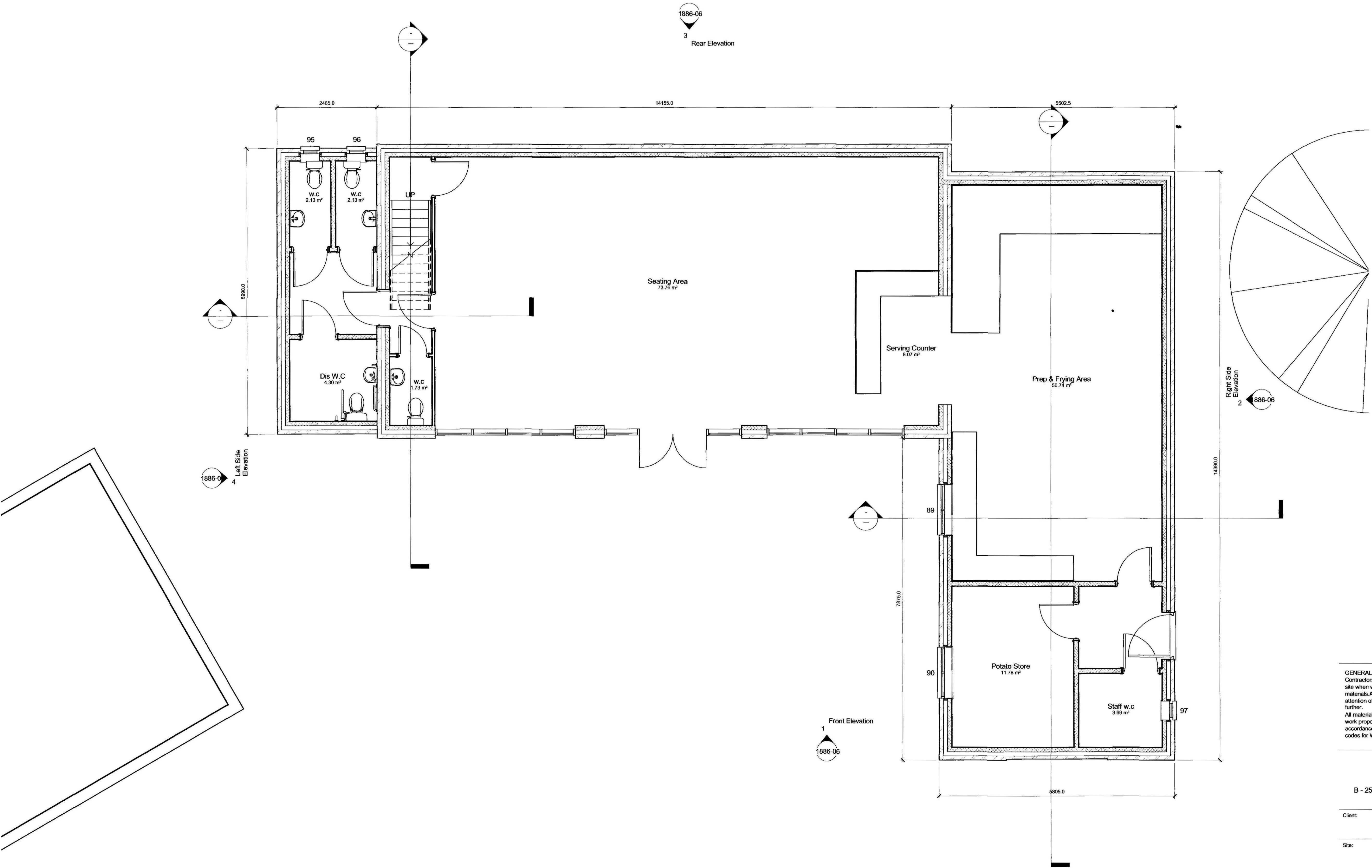
1 Ground Floor 1:50
