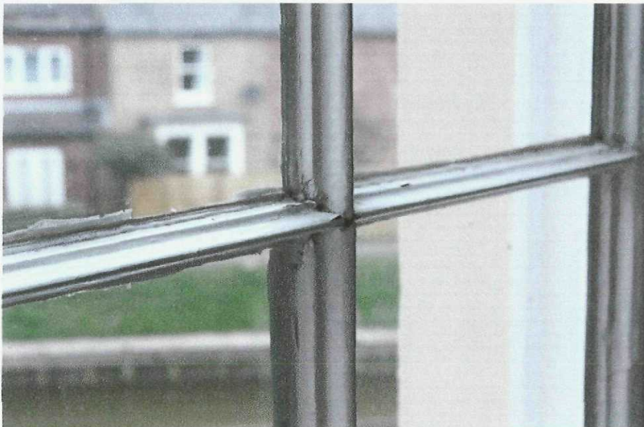
Plate 27: Original window joinery, with lamb's tongue glazing bar profile
