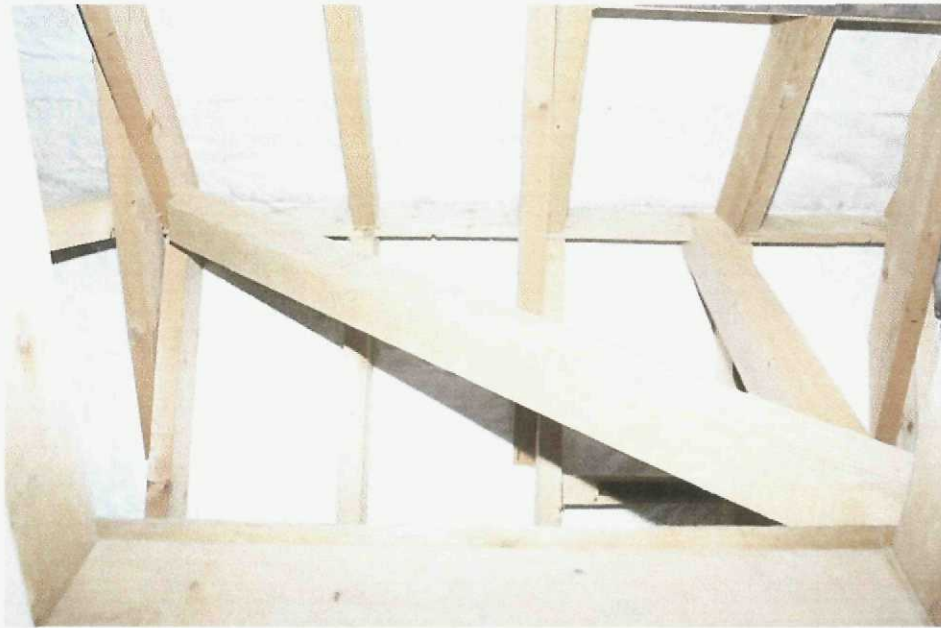
Plate 31: modern softwood roof structure over front, central bay
