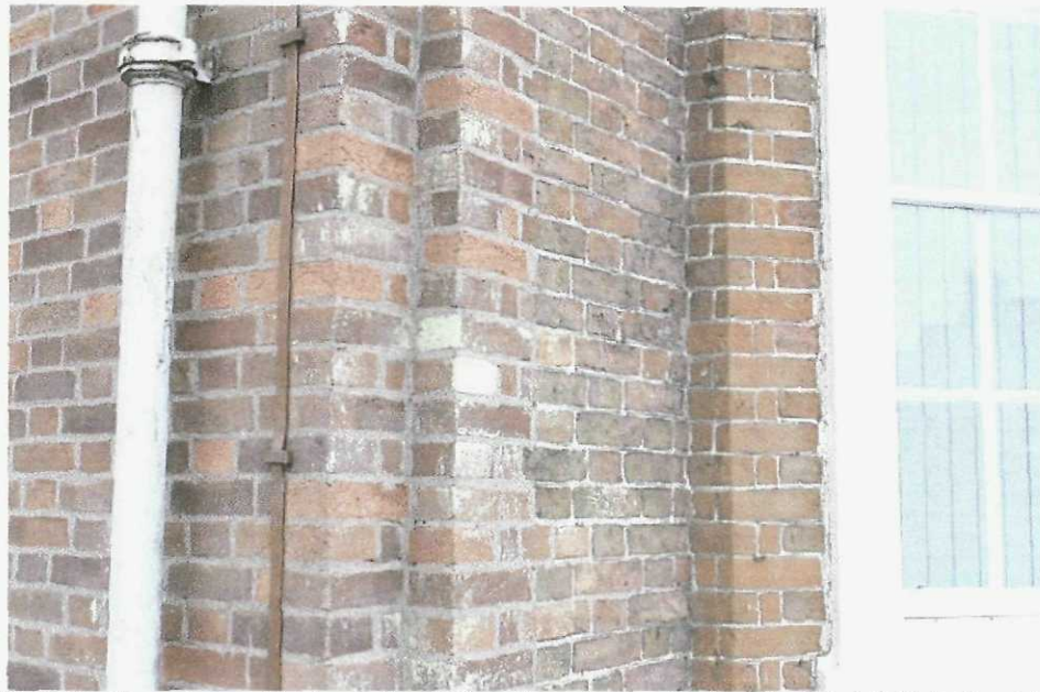
Plate 11: Three phases of brickwork: the c1960 north-east end wall to the left, original 1760s brickwork in the centre, and the later Georgian/early Victorian brickwork of the left-hand front facade canted bay
