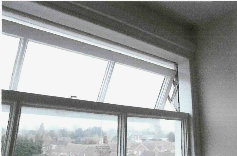
Plate 32: modern outward opening sash to second floor dormer
