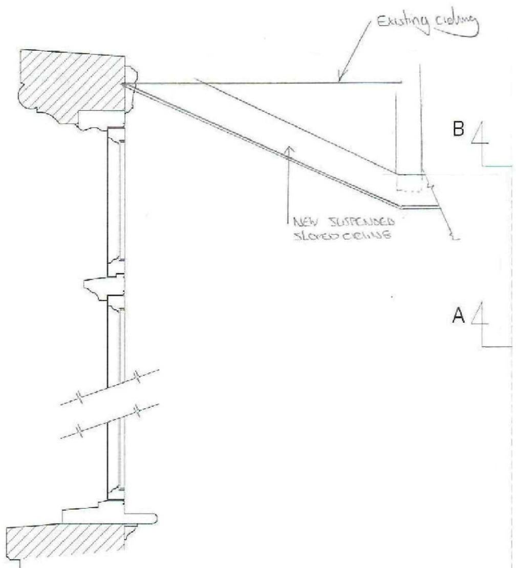
VERTICAL SECTION C-C Scale 1:10
