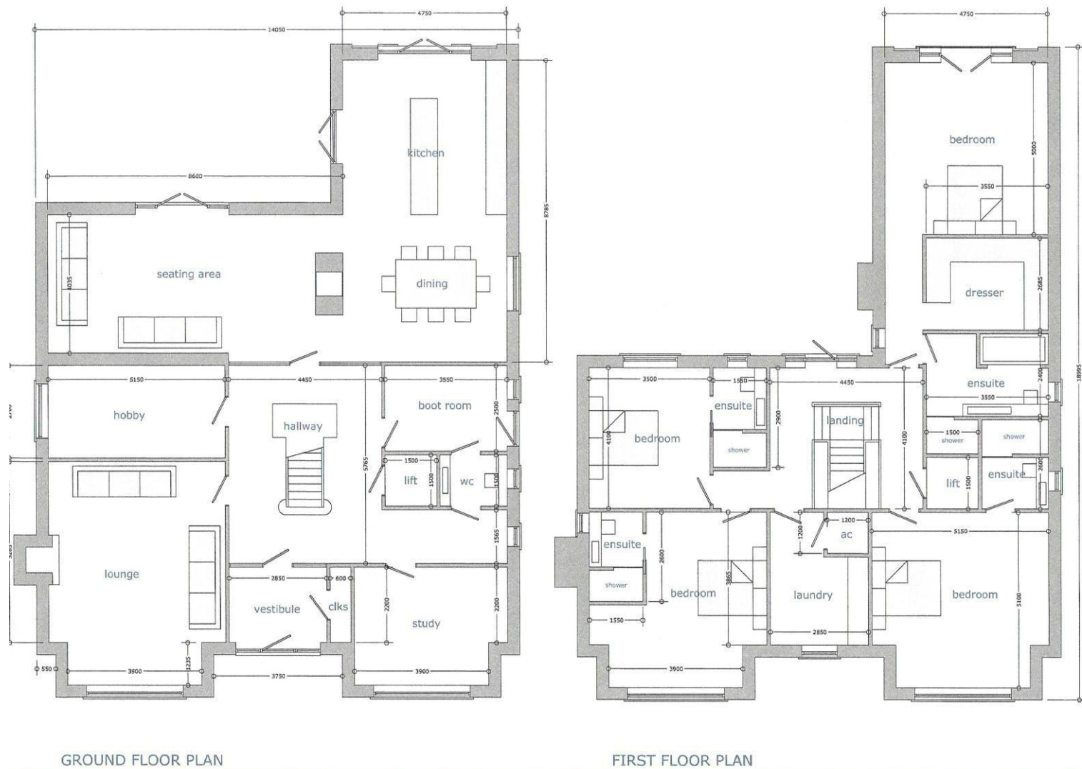
Figure 4: Plan showing the proposed layout of Plot 5 at an original scale of 1:50 at A1, (extract from Architects plan)
