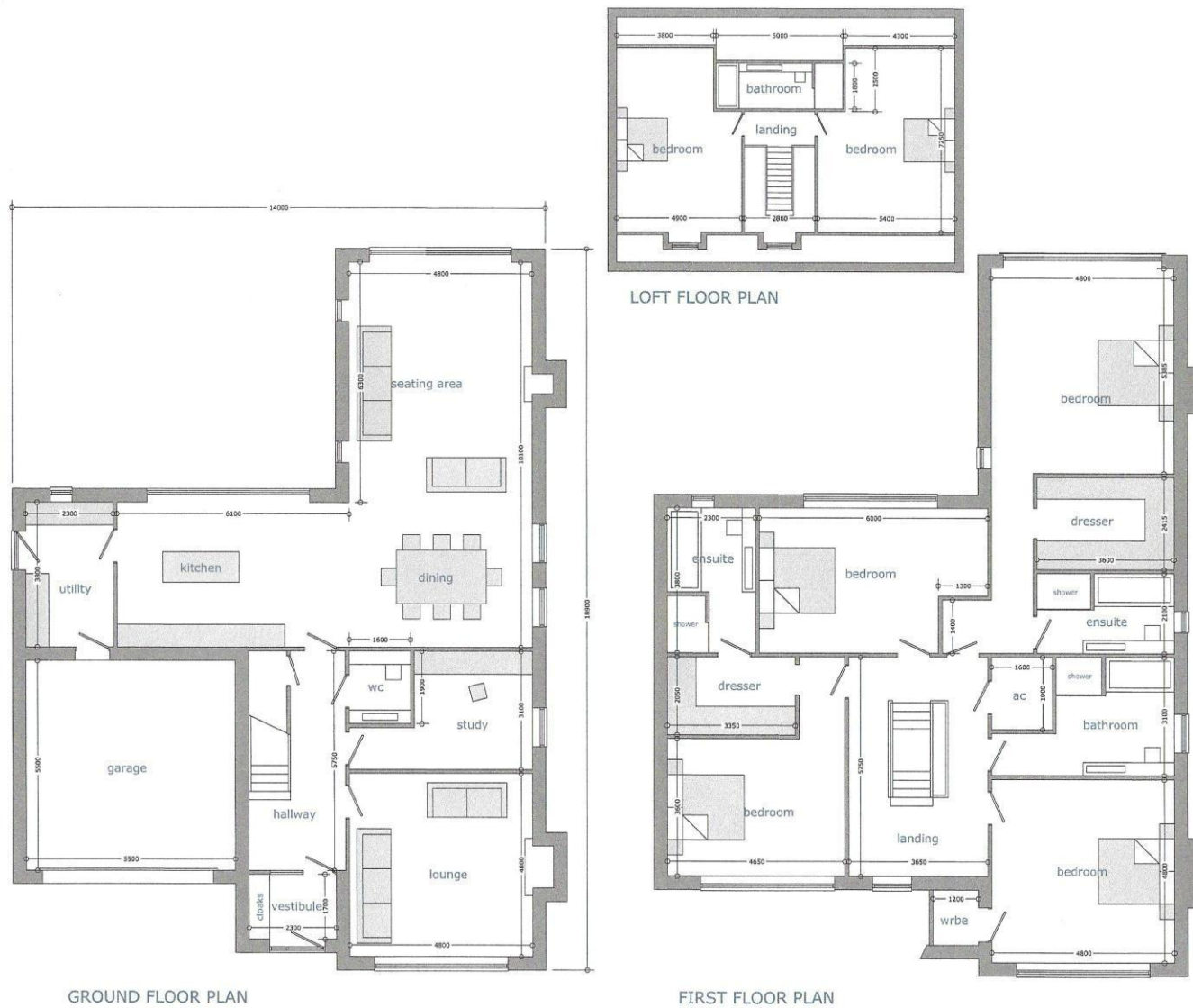
Figure 3: Plan showing the proposed layout of Plot 4 at an original scale of 1:50 at A1, (extract from Architects plan)
