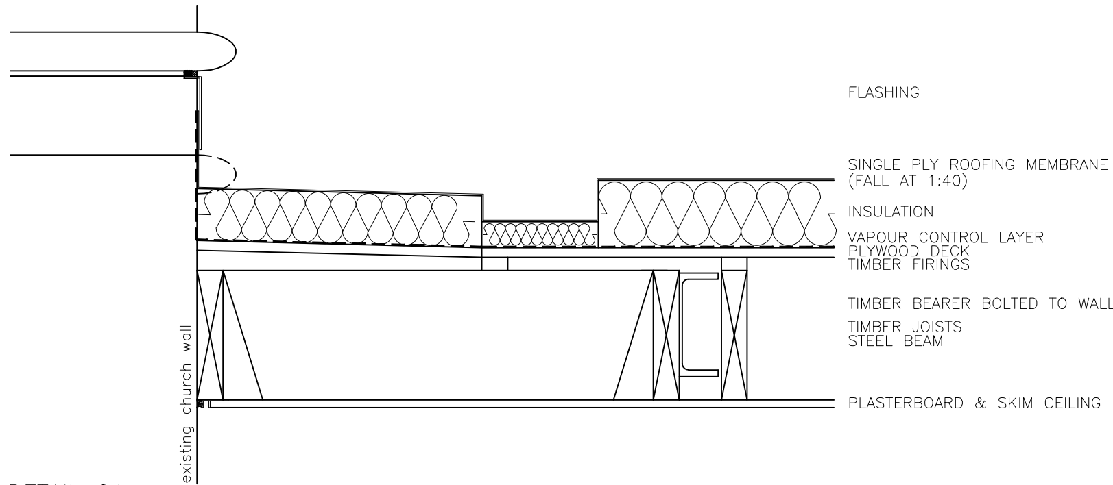
DETAIL 01
