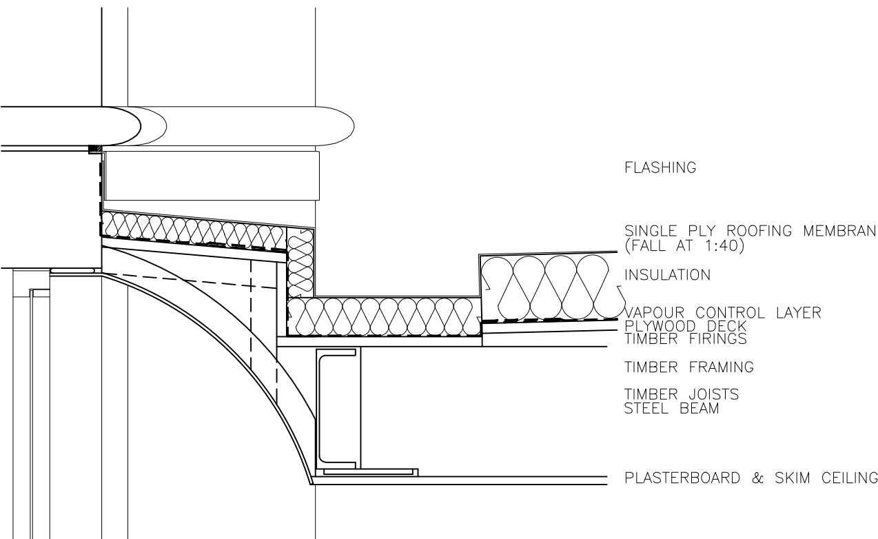
DETAIL 03
