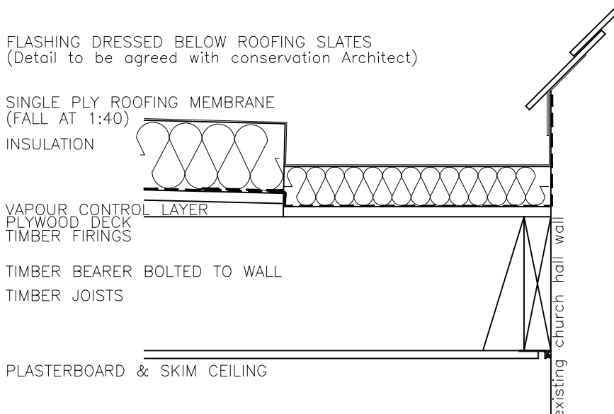
DETAIL 05
