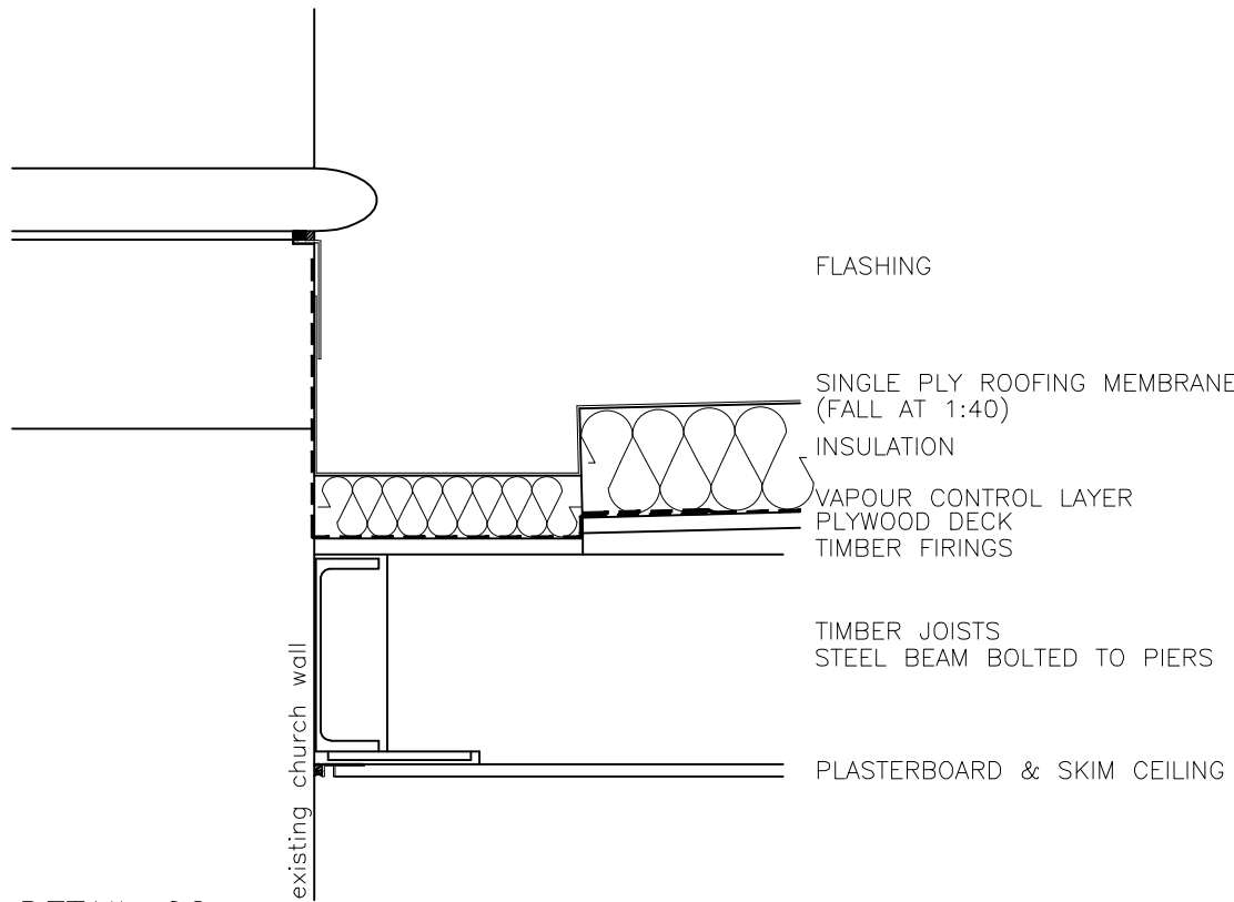
DETAIL 02
