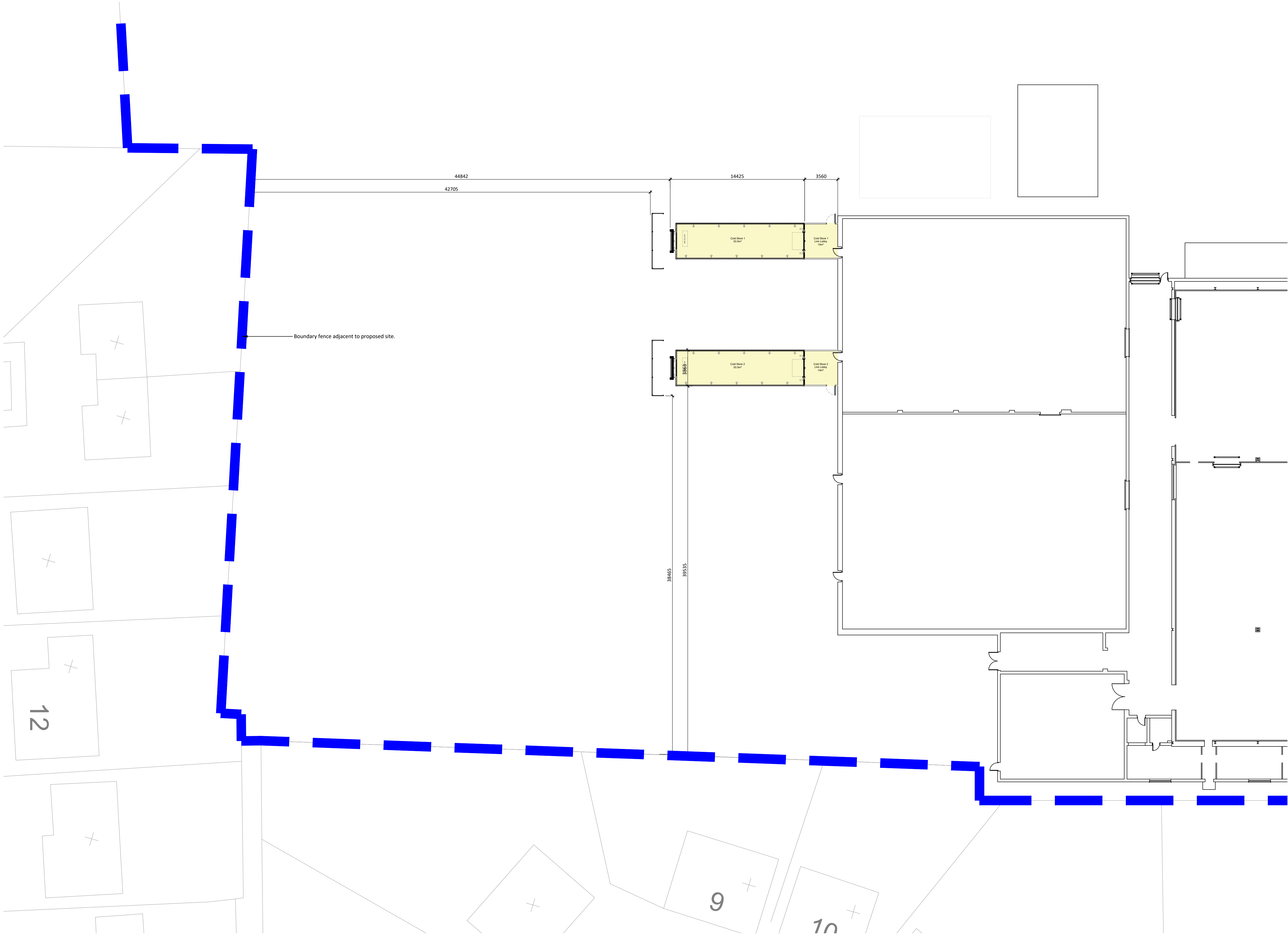
01 Site Boundry Plan P200 SCALE 1:200
