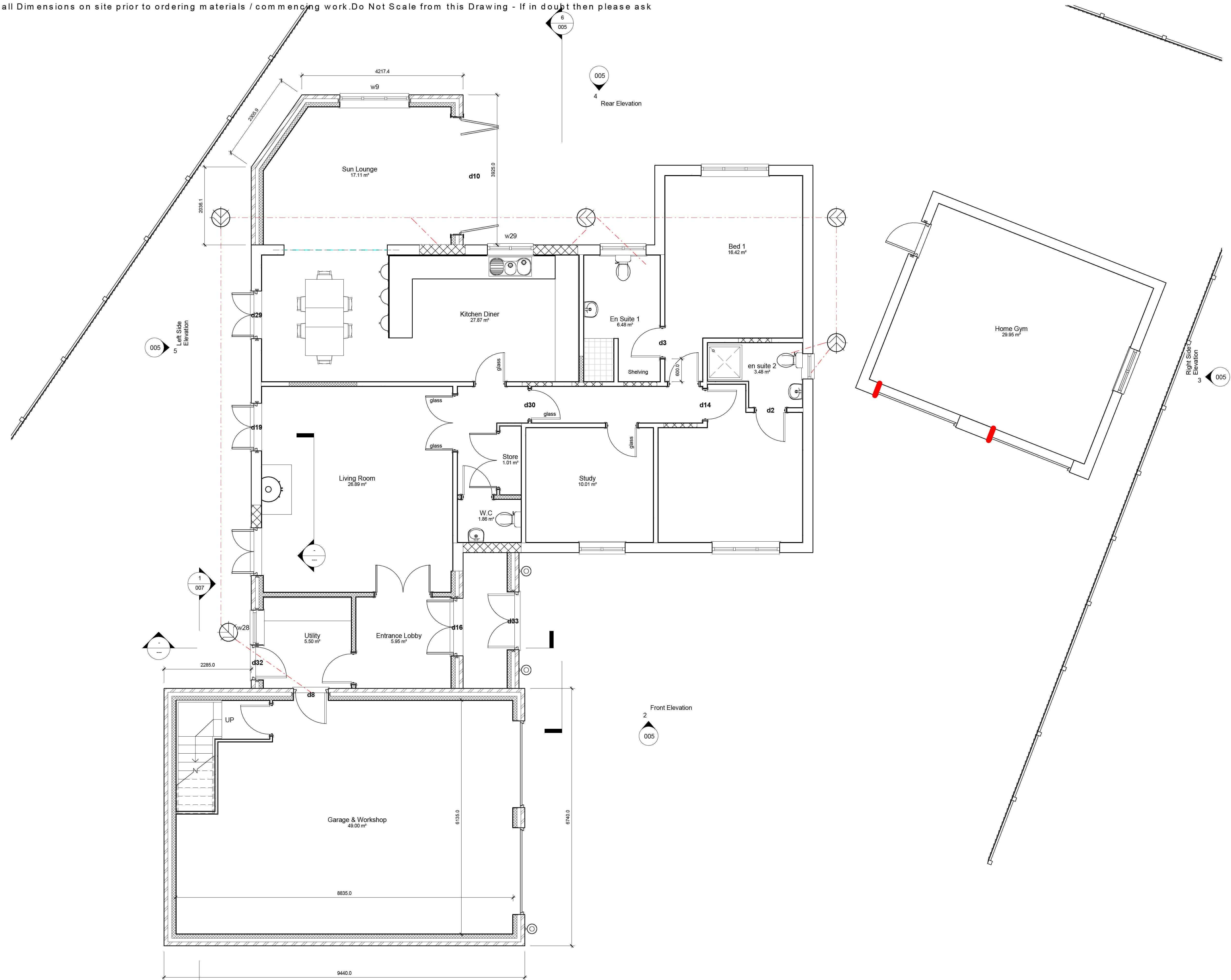
1 Ground Floor 1 : 50
