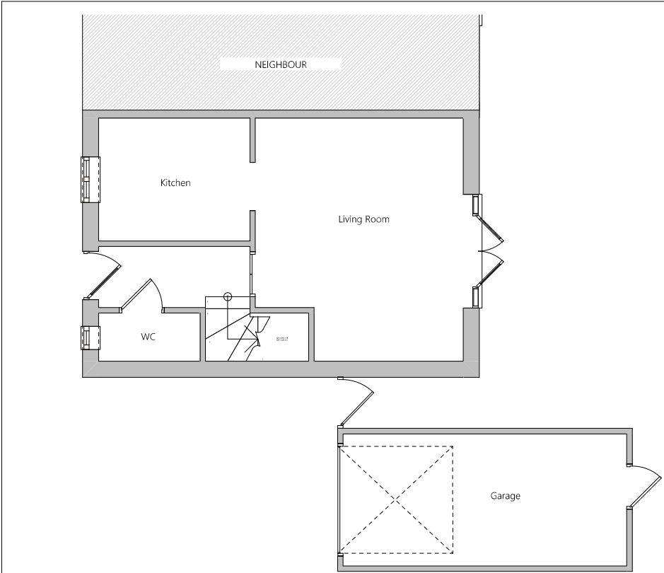
Existing Ground Floor Plan 1:50
