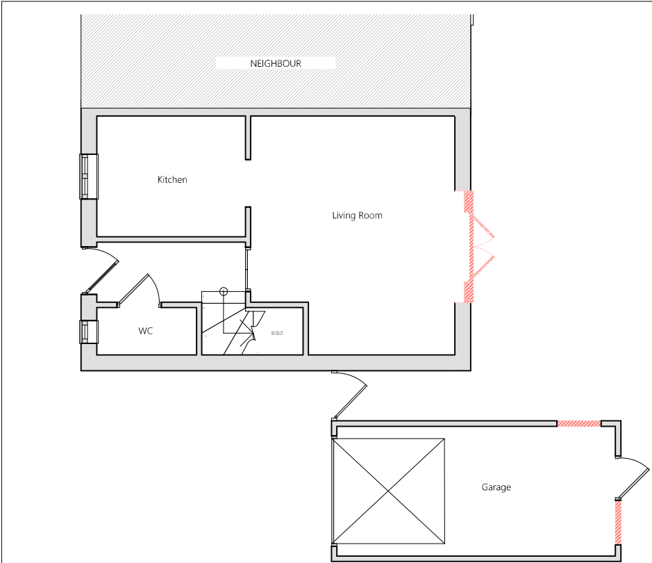
Demolished Ground Floor Plan 1:50
