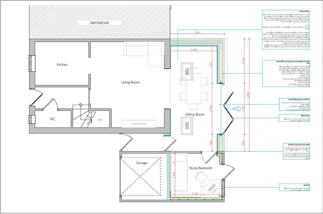
Proposed Ground Floor Plan 1:50 Dimensions to be checked on site by builder.
