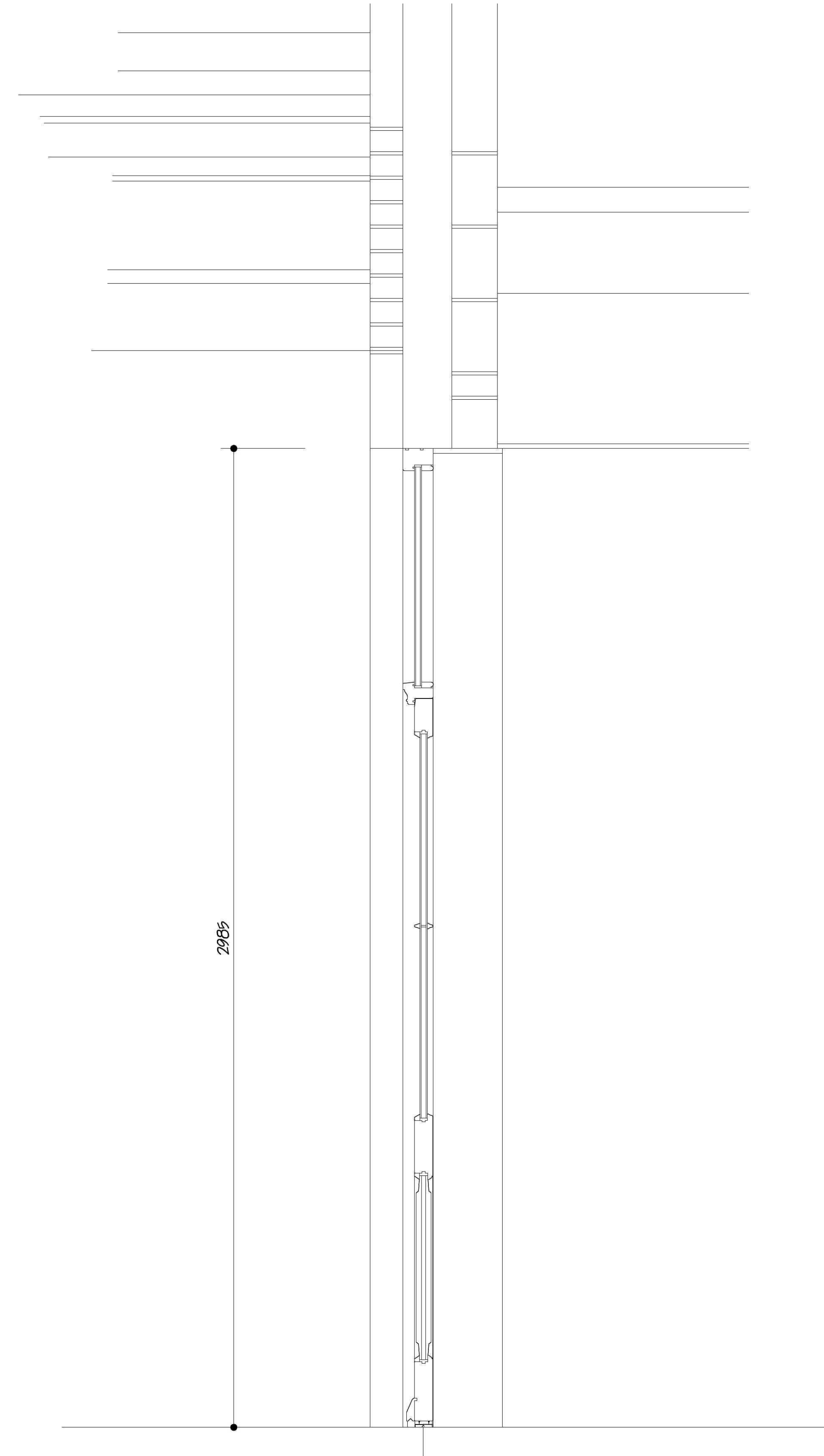
VERTICAL SECTION OF FRENCH DOORS (INWARD OPENING)
