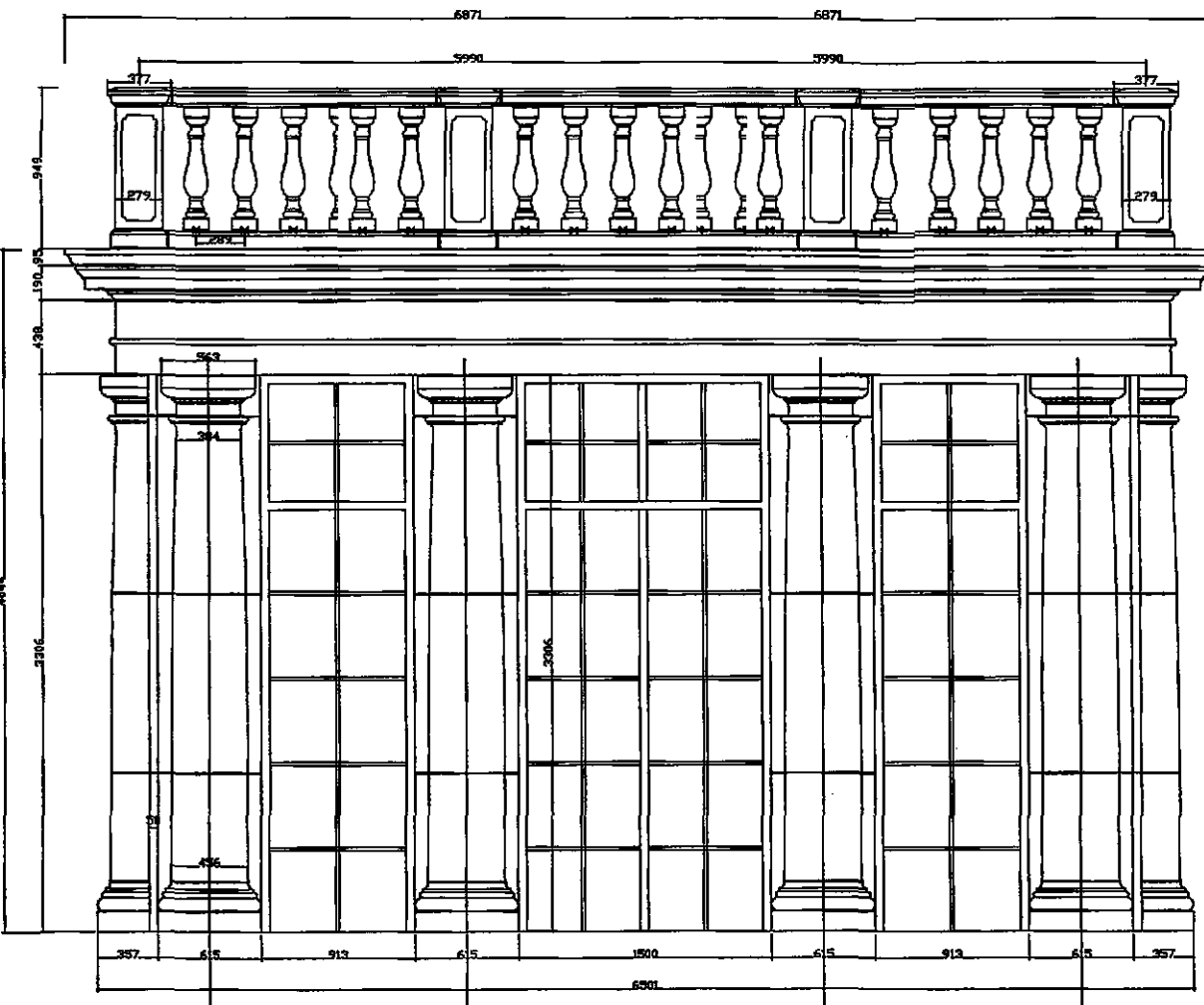
FRONT/END ELEVATION
